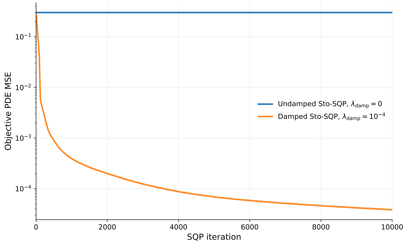
Burgers equation: KKT damping ablation
